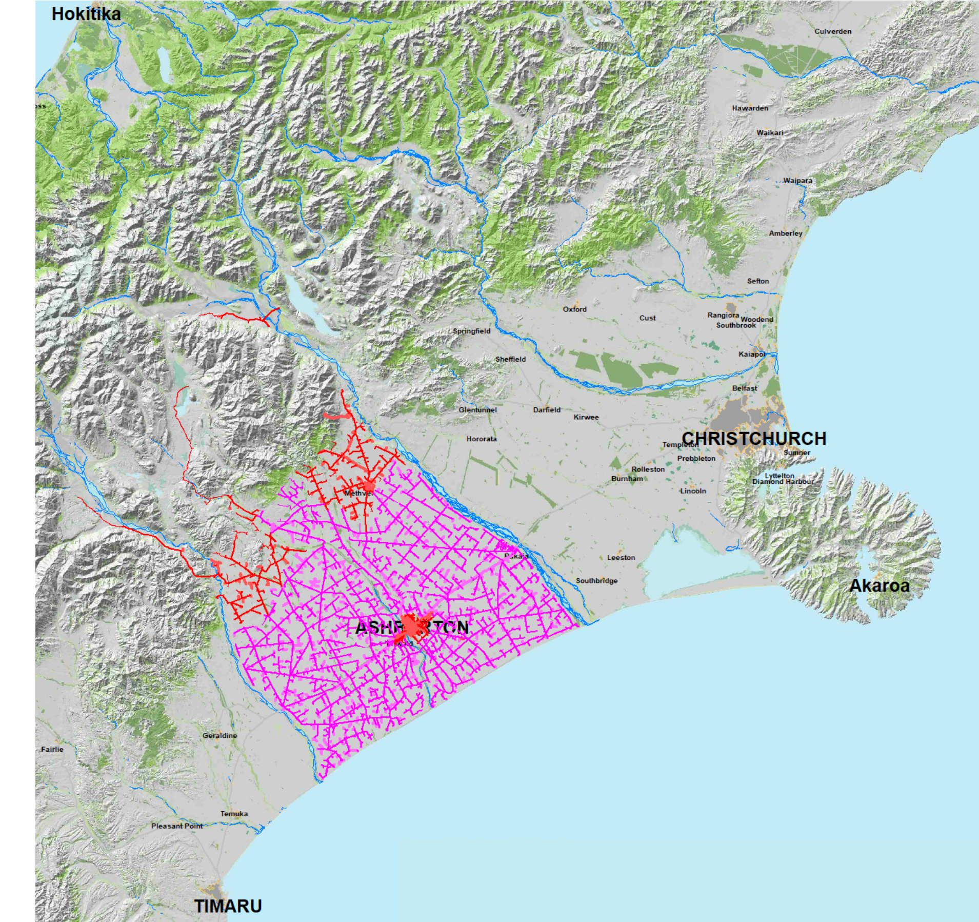
Inset showing EA Networks' location in New Zealand context with 22kV (magenta) and 11kV (red) distribution network. (OA), (OB), (OD), (OF), (OI), (A), (C), (E), & (G)
